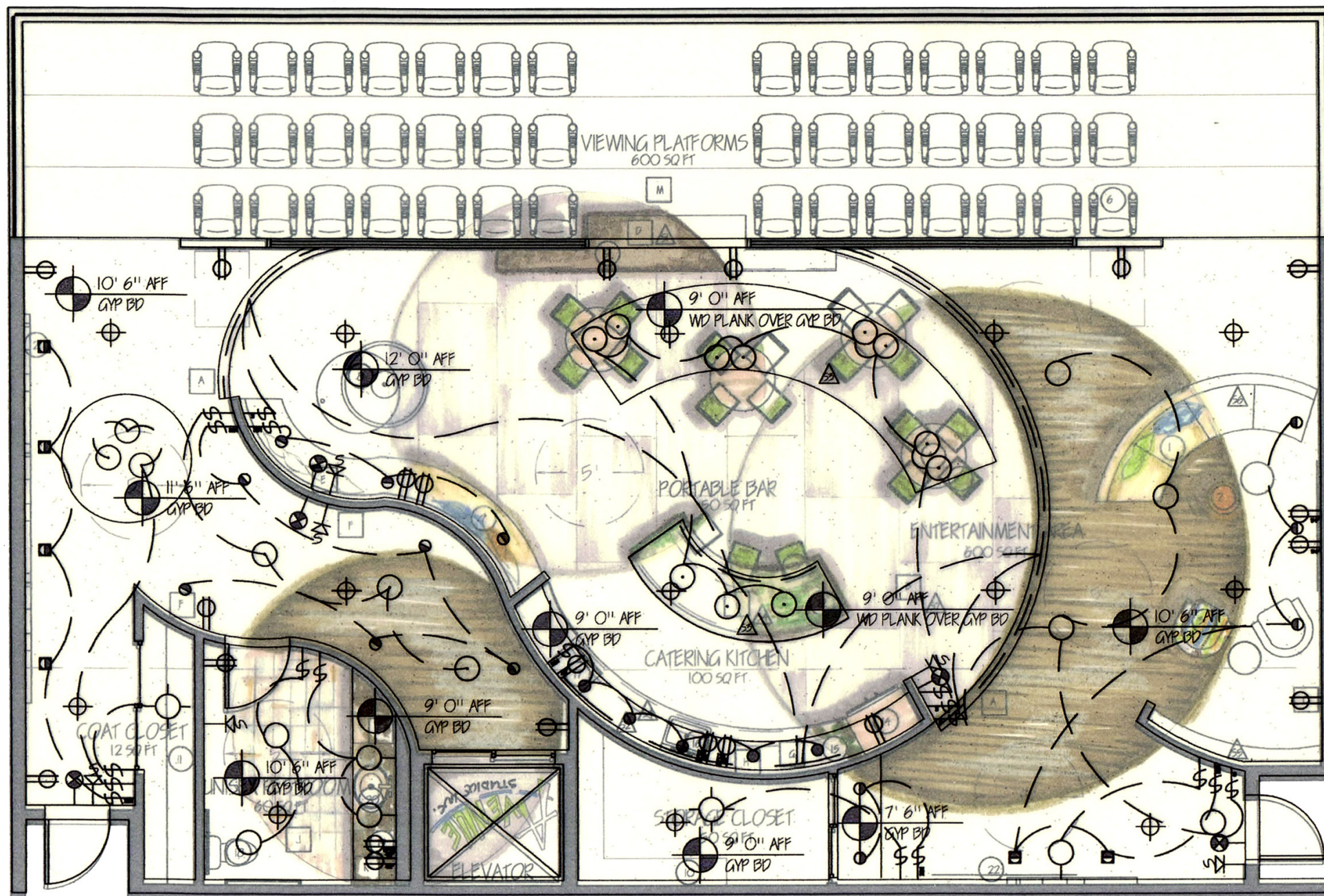
Reflected Ceiling Plan with Switching Diagram
